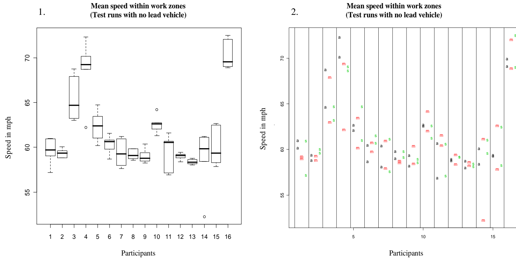
Figure C4 – Mean speeds within work zones in test runs without lead vehicles
